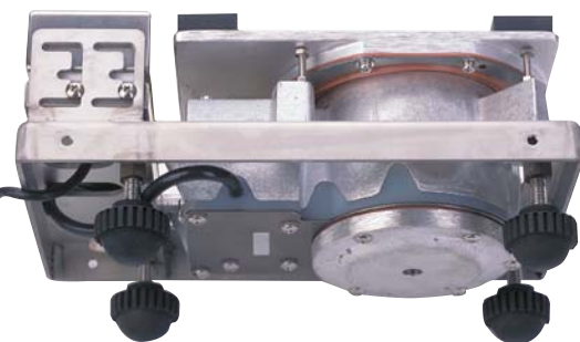
Hermetically sealed load cell
